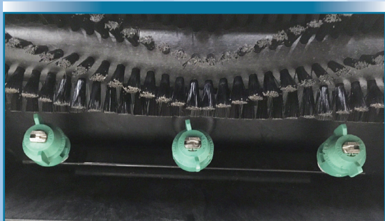
Three long-lasting, stainless steel, twist-lock spray jets, and a stainless steel vacuum shoe
